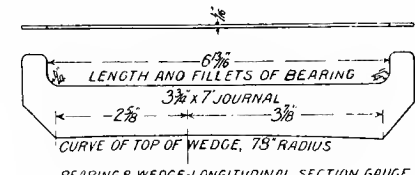
BEARING & WEDGE LONGITUDINAL SECTION GAUGE
